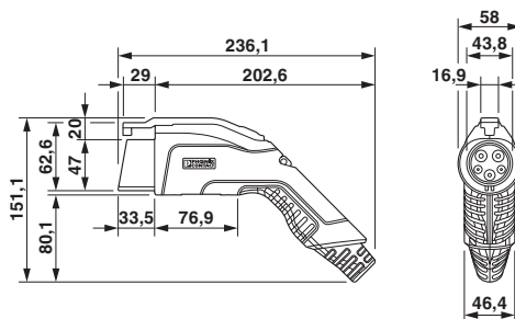
Vehicle connector
